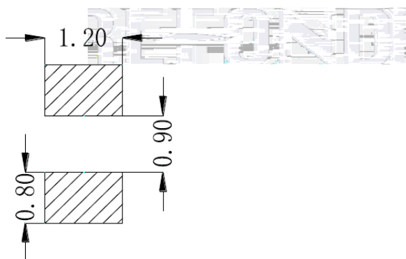
Fig.1-5 Soldering Patterns
