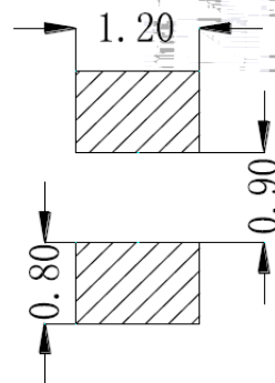
Fig.1-5 Soldering Patterns
