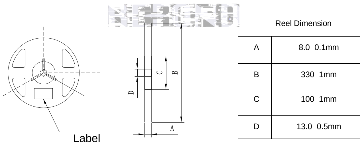
Fig.2-2 Reel Dimension
