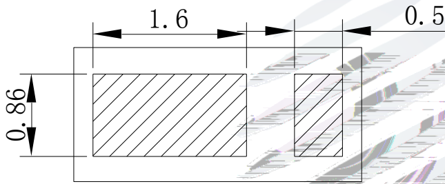
Fig.1-3 Bottom View
