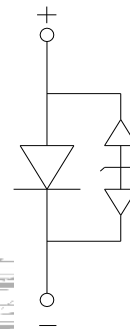
Fig.1-4 Polarity
