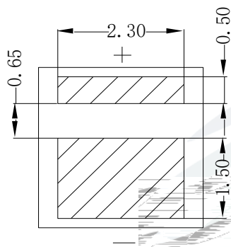
Fig.1-3 Bottom View
