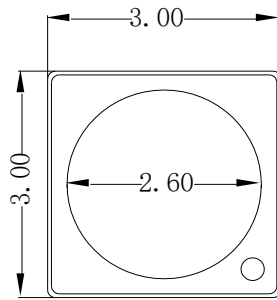
Fig.1-1 Top View
