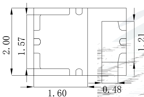
Fig.1-3 Bottom View
