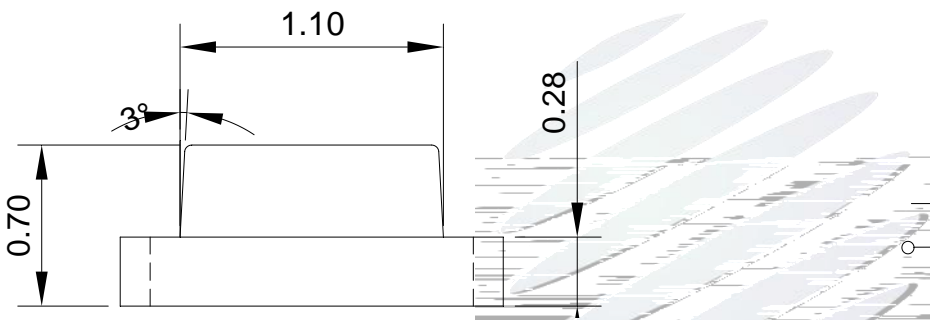
Fig.1-3 Side view
