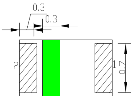
Fig.1-3 Bottom view
