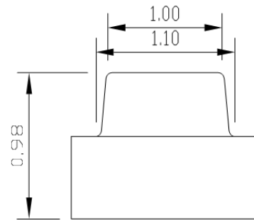
Fig.1-2 Side view
