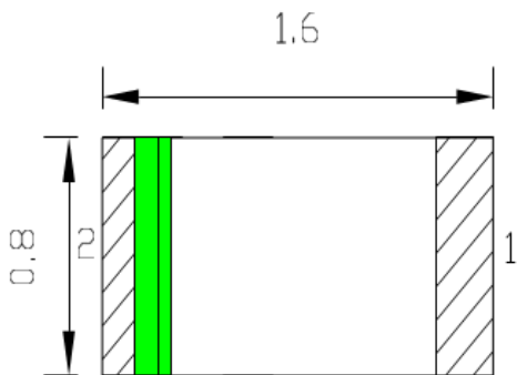
Fig.1-1 Top view
