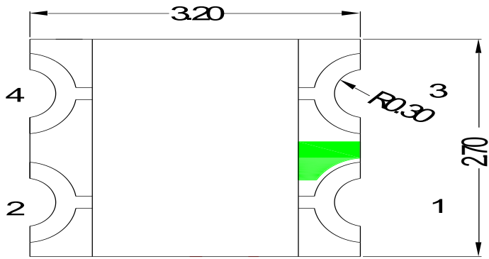
Fig.1-1 Top view
