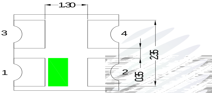
Fig.1-3 Bottom view
