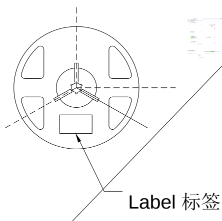
Fig.2-2 Reel Dimension
