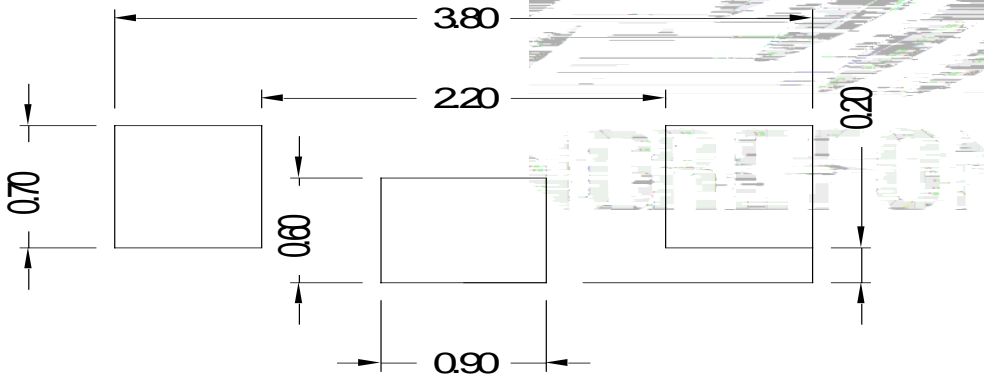
Fig.1-5 Soldering patterns
