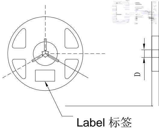
Fig.2-2 Reel Dimension
