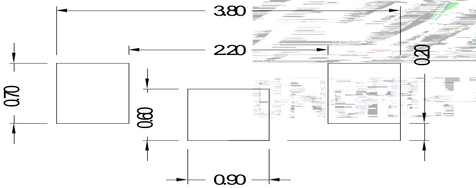
Fig.1-5 Soldering patterns
