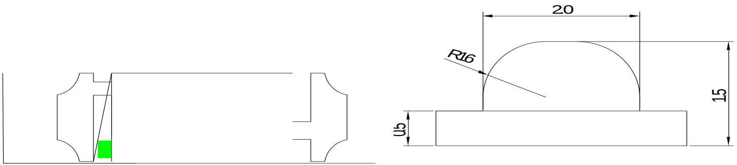
Fig.1-1 Top view
