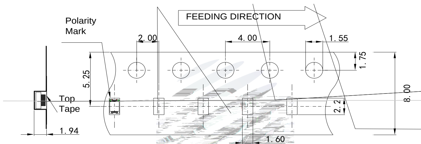
Fig.2-1 Carrier Tape Dimension 載帶尺寸
