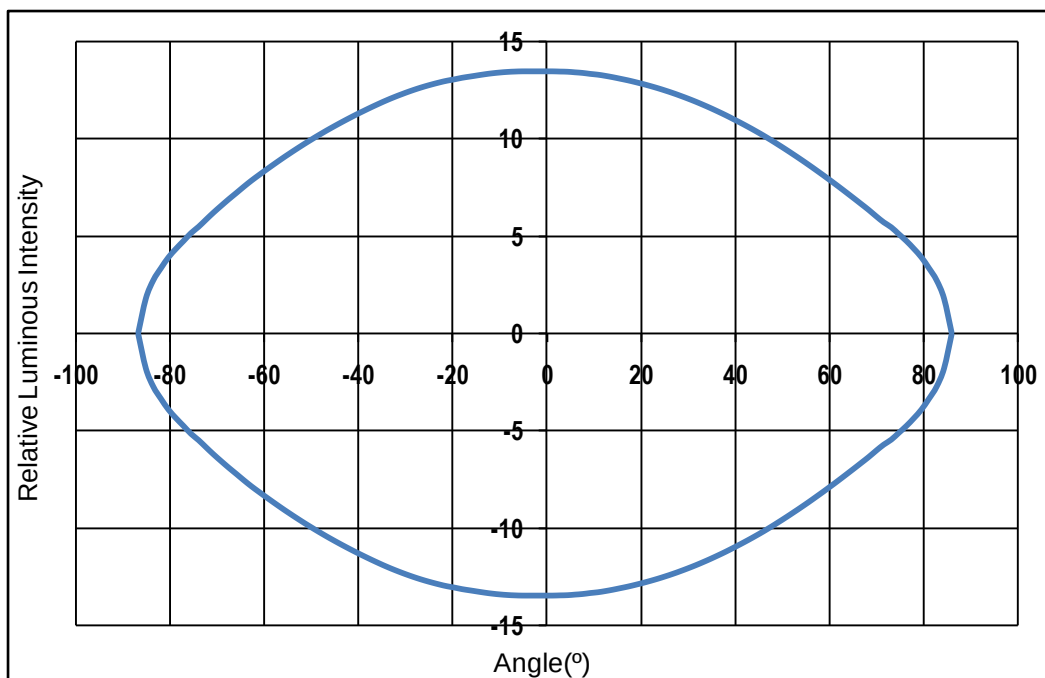
Fig. 1-11 Radiation diagram
