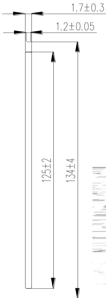
Fig.1-1 Top view
