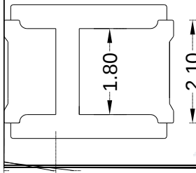
Fig.1-3 Bottom view
