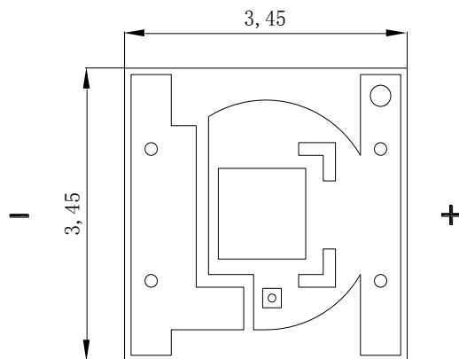
Fig.1-1 Top view
