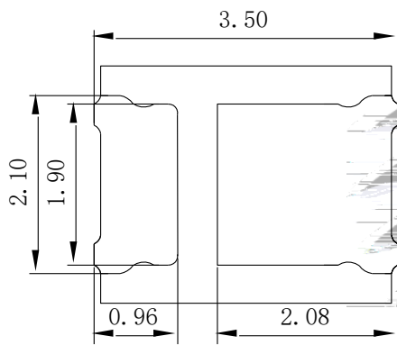
Fig.1-3 Bottom view
