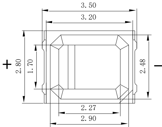
Fig.1-1 Top view
