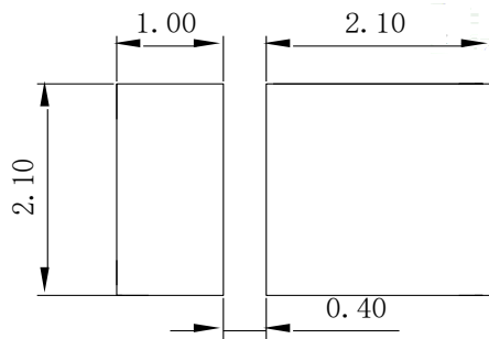
Fig.1-5 Soldering patterns
