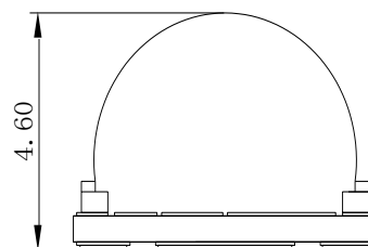
Fig.1-2 Side view
