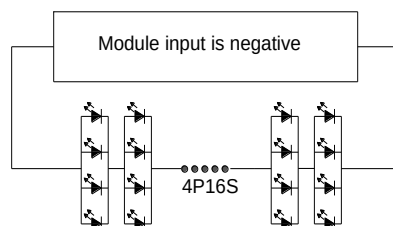
Fig.2-2ED Module connection
