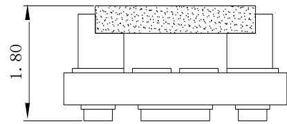
Fig.1-2 Side view
