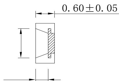
Fig.1-2 Side view 侧面视图
