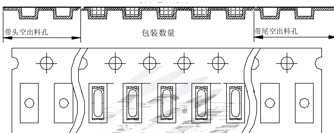
Fig 2-1 Carrier Tape Dimensions 载带尺寸
