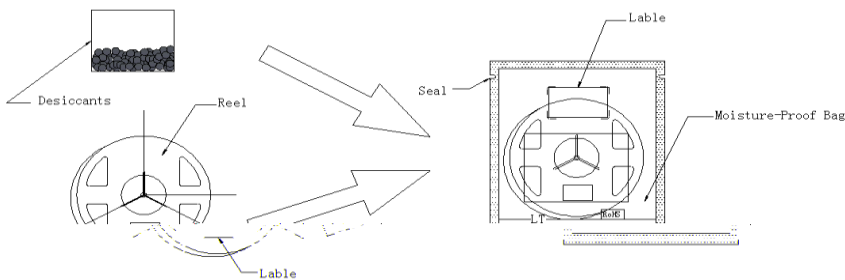
Fig.2-4 Moisture Resistant Packing
