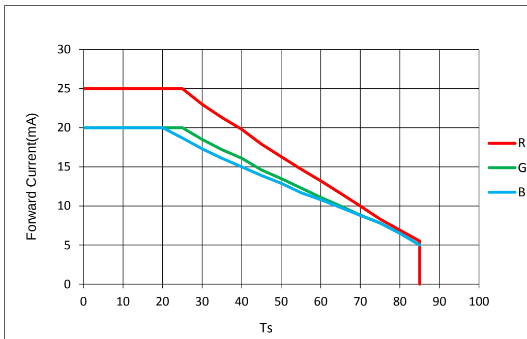
Fig 1-9 Solder Temperature Vs Forward Current 回流焊温度与正向电流特性曲线
