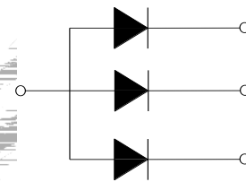
Fig.1-4 Polarity
