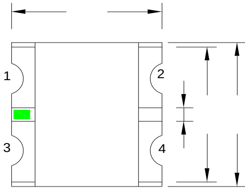
Fig.1-1 Top view
