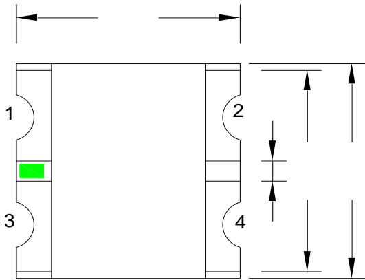
Fig.1-1 Top view
