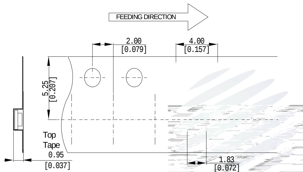
Fig.2-1 Carrier Tape Dimension
