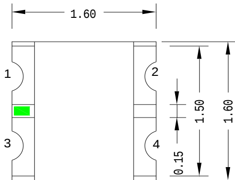
Fig.1-1 Top view
