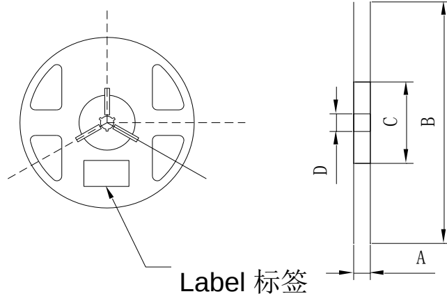
Fig.2-2 Reel Dimension
