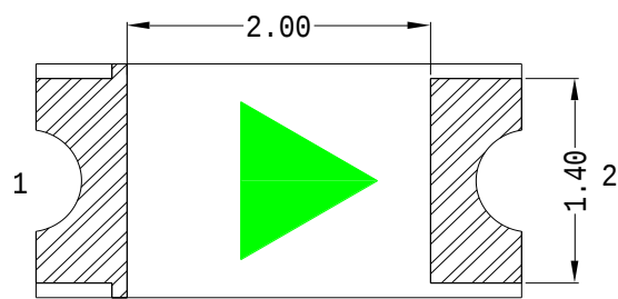
Fig.1-2 Bottom view
