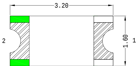
Fig.1-1 Top view
