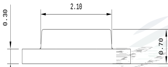
Fig.1-3 Side view
