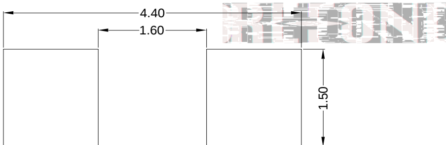
Fig.1-5 Soldering patterns
