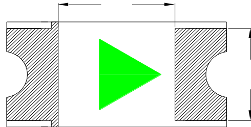
Fig.1-2 Bottom view
