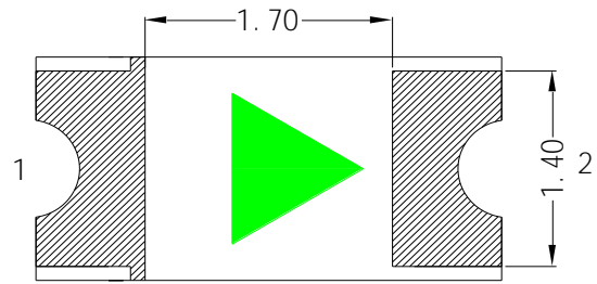
Fig.1-2 Bottom view
