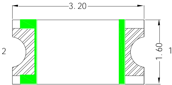
Fig.1-1 Top view
