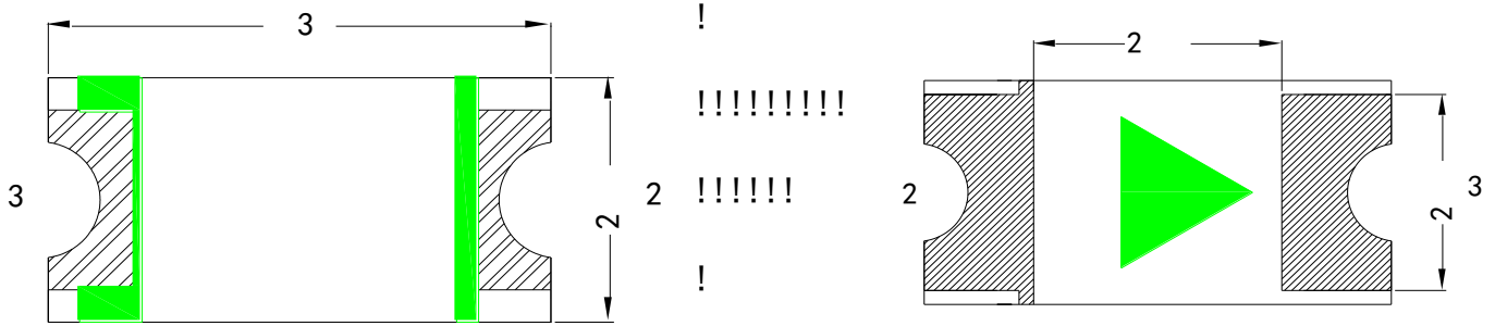
Fig.1-1 Top view!
