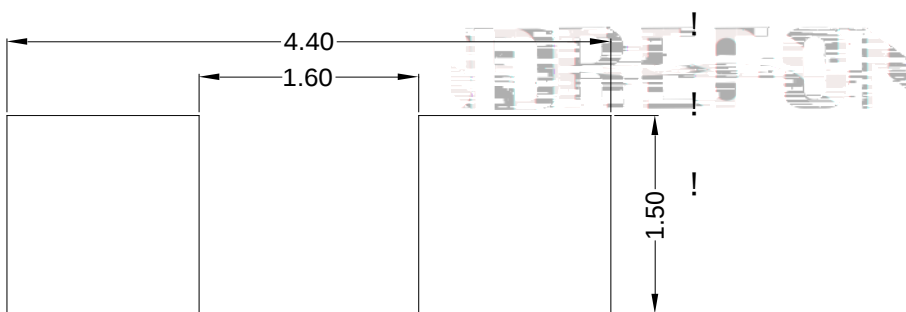
Fig.1-5 Soldering patterns!
