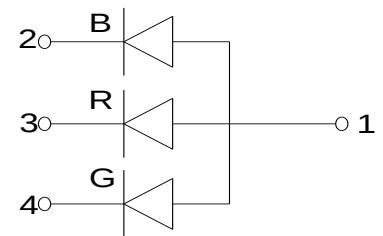
Fig.1-4 Polarity
