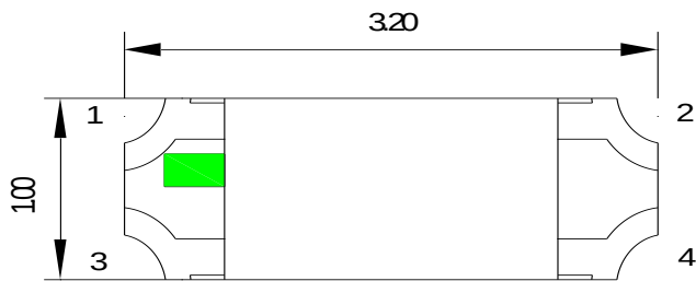
Fig.1-1 Top view
