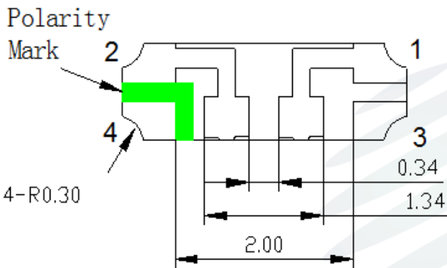
Fig.1-3 Bottom view
