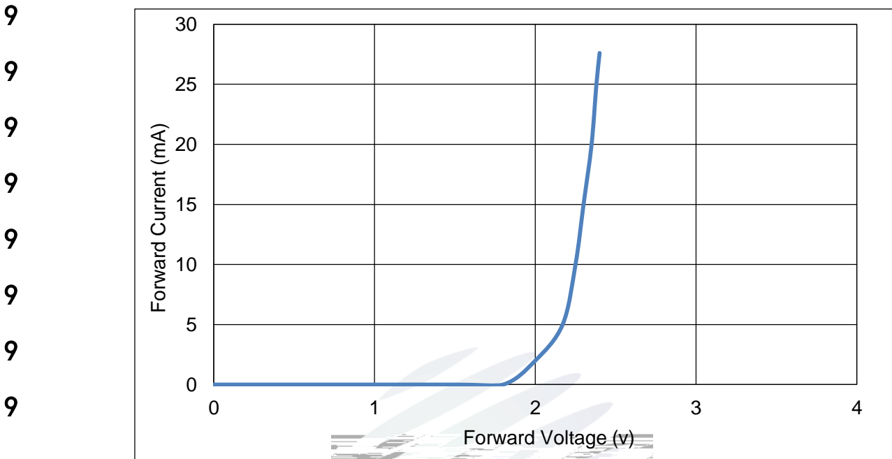
Fig 1-6 Forward Voltage Vs Forward Current
