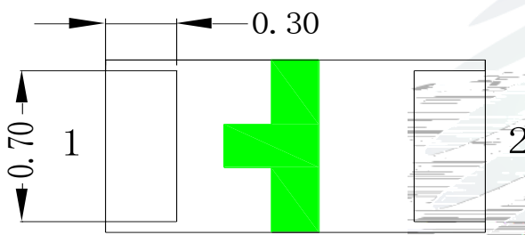
Fig.1-3 Bottom view
