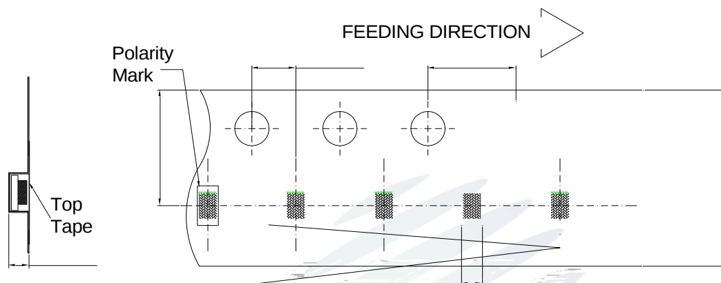
Fig.2-1 Carrier Tape Dimension
