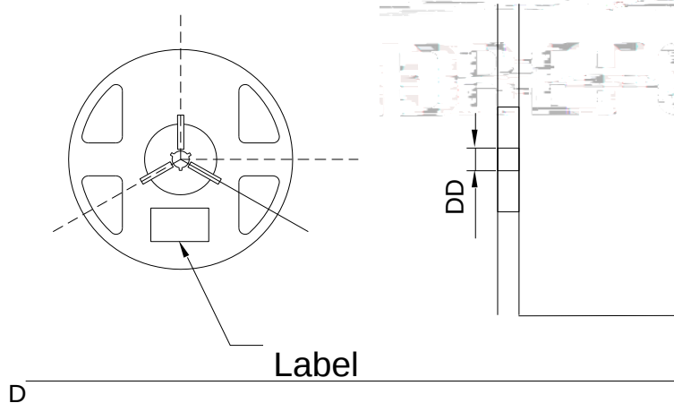
Fig.2-2 Reel Dimension
