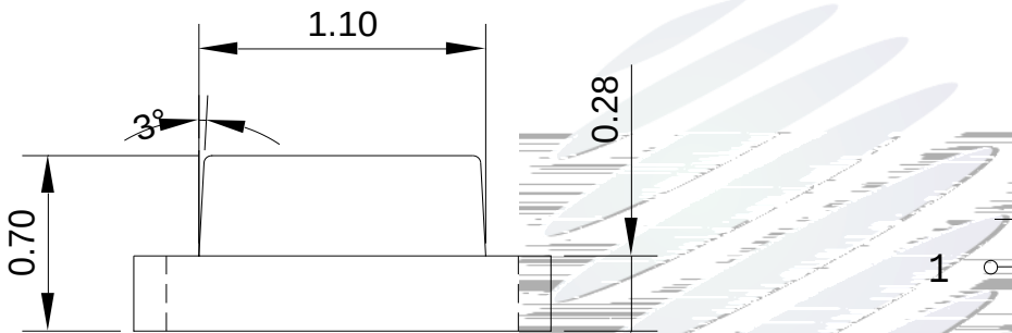
Fig.1-3 Side view
