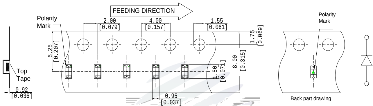
Fig.2-1 Carrier Tape Dimension
