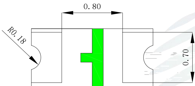
Fig.1-3 Bottom view
