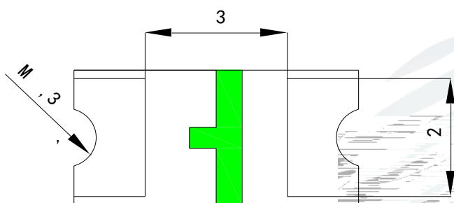
Fig.1-3 Bottom view
