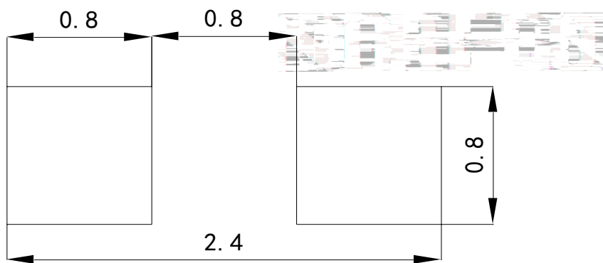
Fig.1-5 Soldering patterns
