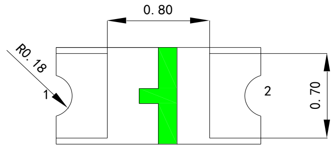
Fig.1-2 Side view
