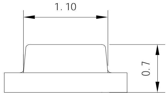
Fig.1-2 Side view
