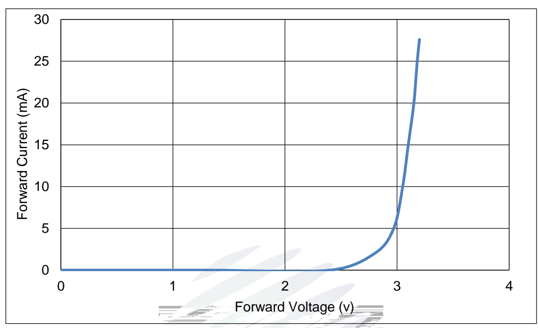
Fig 1-8 Forward Voltage Vs Forward Current
