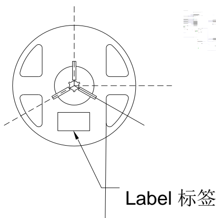
Fig.2-2 Reel Dimension
