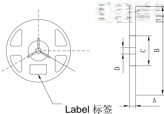
Fig.2-2 Reel Dimension
