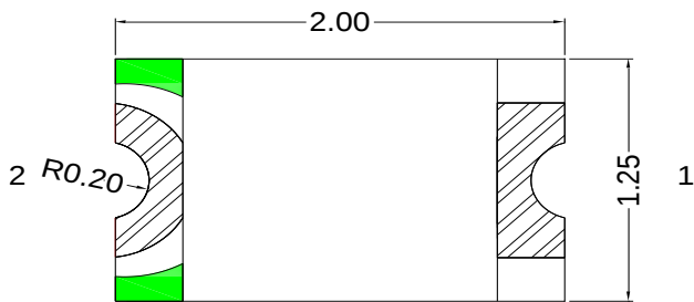
Fig.1-1 Top view
