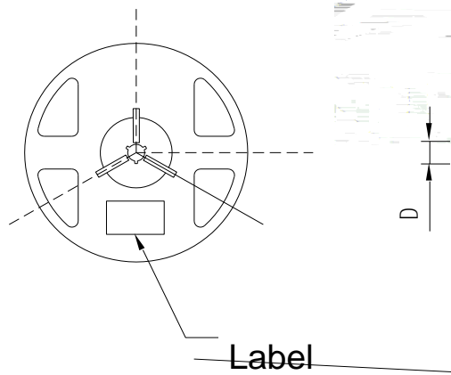
Fig.2-2 Reel Dimension
