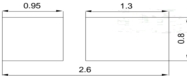
Fig.1-3 Bottom view
