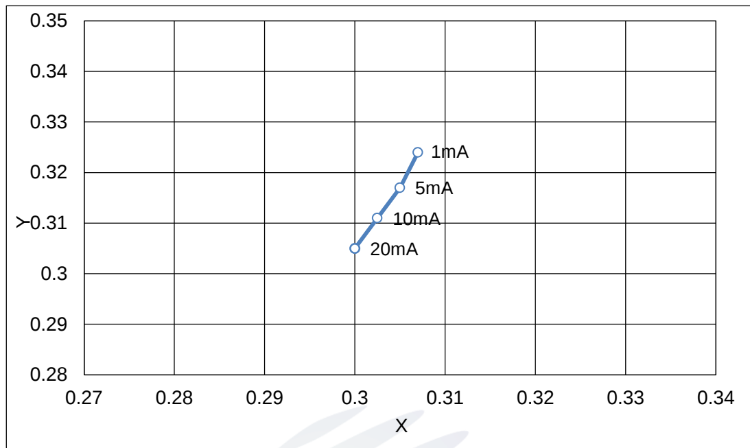
Fig. 1-11 Forward Current Vs Dominate Wavelength ( T_a=25^\circ\text{C} )
