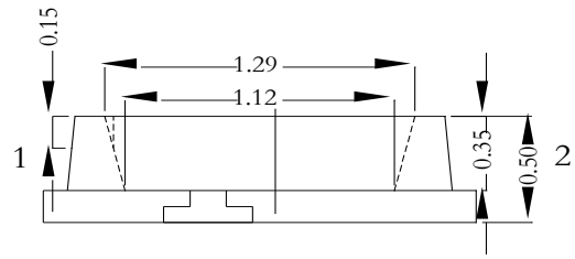
Fig.1-2 Side view
