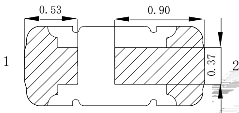
Fig.1-3 Bottom view
