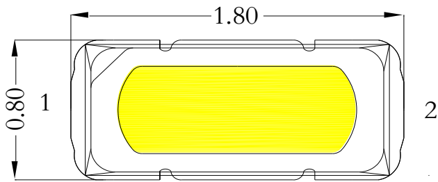
Fig.1-1 Top view
